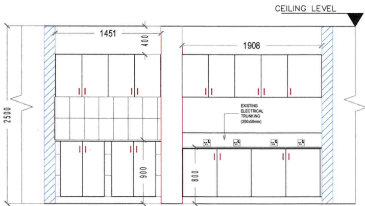
EXISTING ELEVATION - A 18th November 2024
