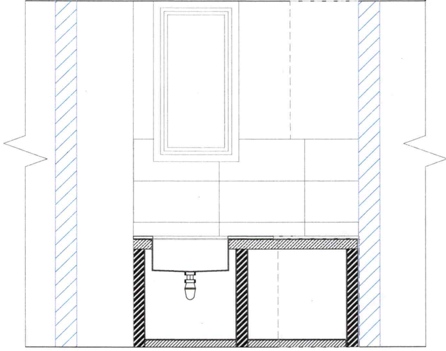
PROPOSED SECTION X-X
