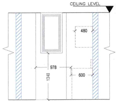
EXISTING ELEVATION - B 18th November 2024
