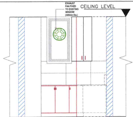
PROPOSED ELEVATION - B
